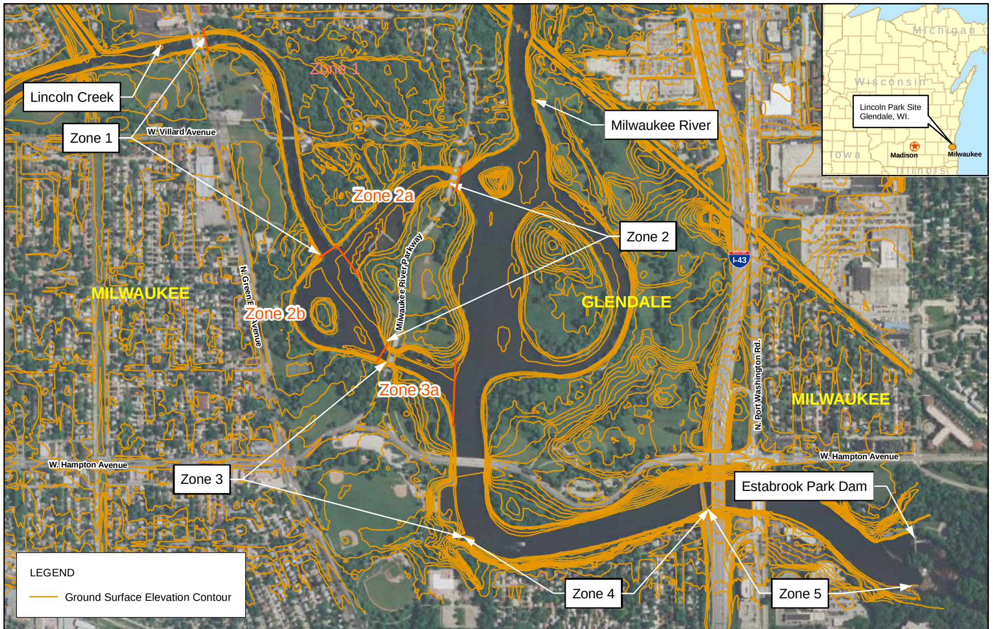
Figure 5 Lincoln Park Site Topographic Contour Lines Feasibility Study Glendale, WI
